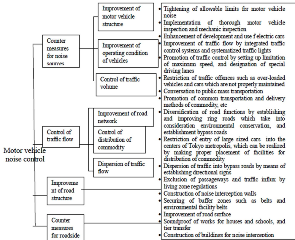
Fig. 10.1: Control Scheme for Motor Vehicle Noise Pollution
